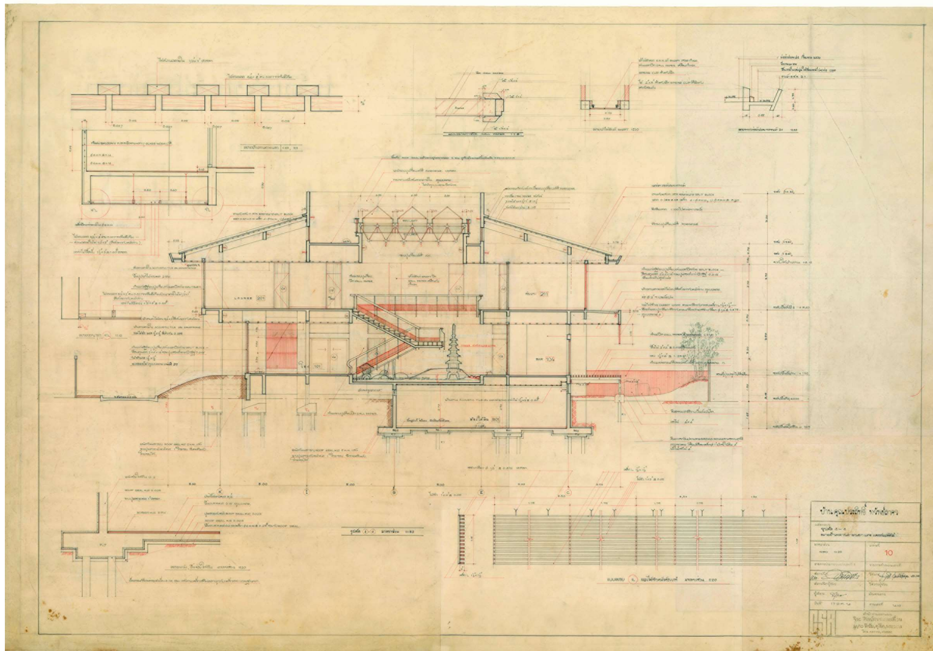
House for Mr Prasit Sapsakhon, Chira Silpakanok, 1969
