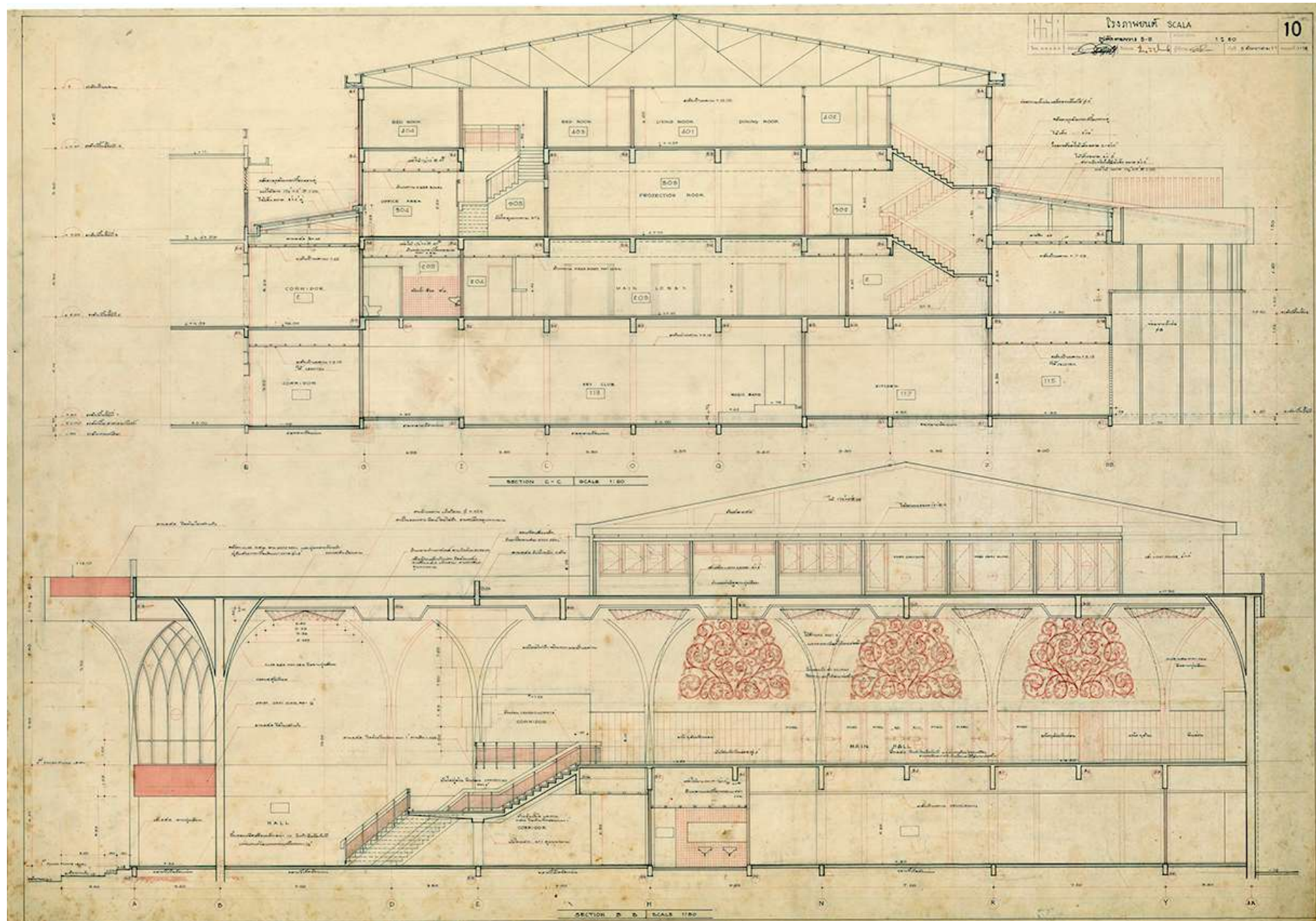
Scala Cinema, Chira Silpakanok, 1971
